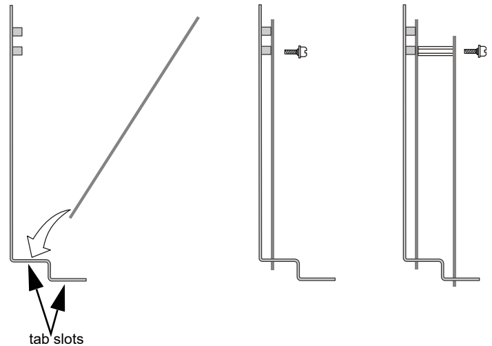
Figure 2 Installing IDP/SK Multi-Modules
