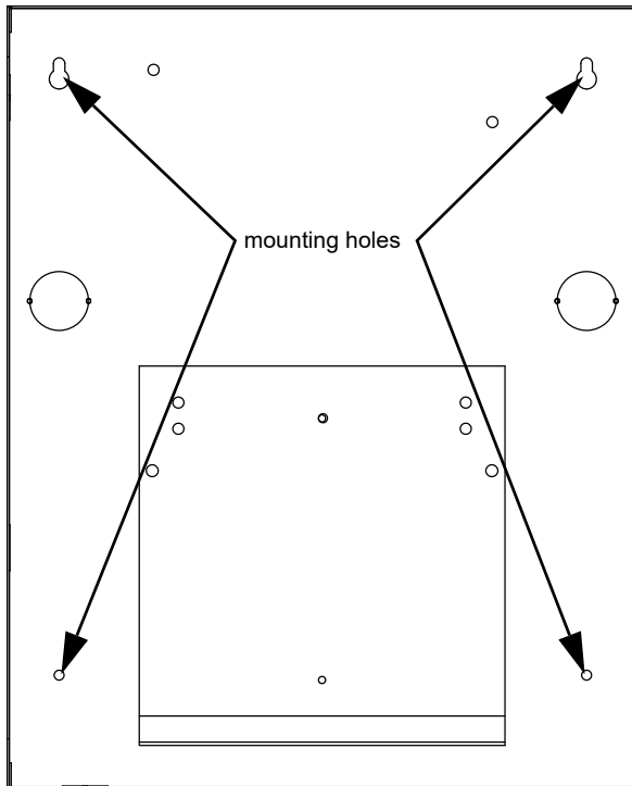
Figure 1 Mounting the IDP-ACB
