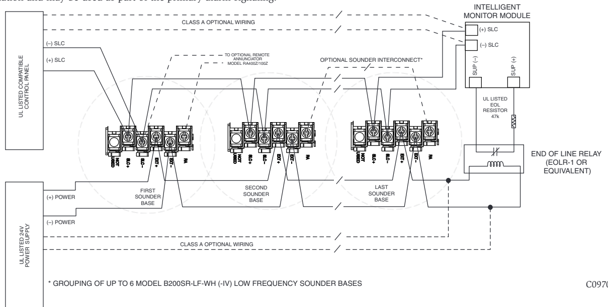
FIGURE 6: WIRING DIAGRAM
