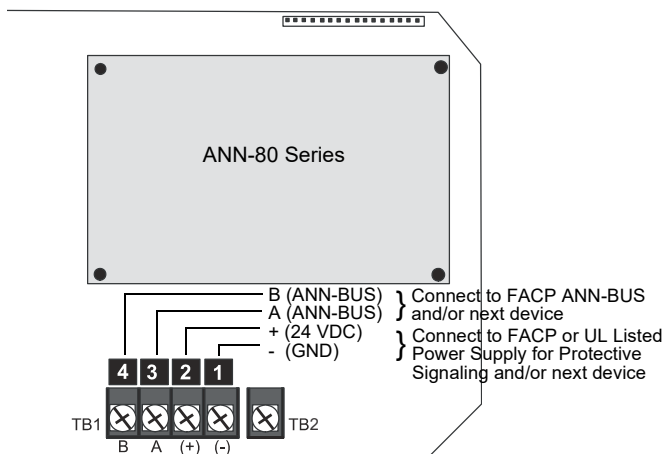
Figure 3 Wiring the ANN-80(-W) to an FACP
