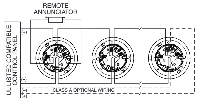
FIGURE 1. WIRING DIAGRAM
