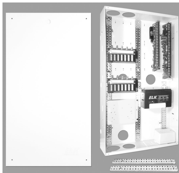
ELK-SWB pictured with optional Security Control, Automation Controller, and typical Telco/CATV module.
