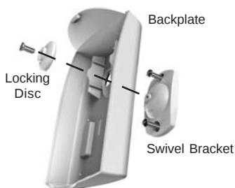
Figure 4. Standard Swivel Mounting
