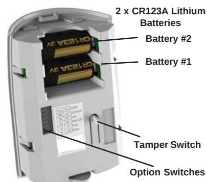
Figure 5. Back View of Sensor
