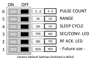
Figure 7. DIP Switches
