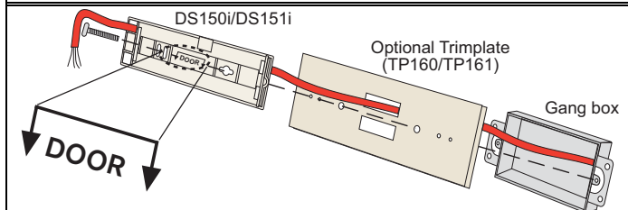
Figure 1: Optional Trimplate
