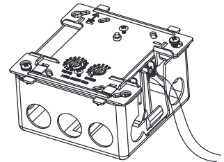
FIGURE 2A. MODULE MOUNTING WITH BARRIER:
