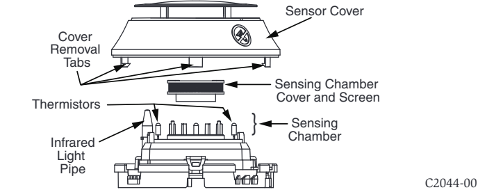
FIGURE 4. CLEANING THE FIRE/CO DETECTOR
