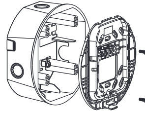
3D. CEILING MOUNT SURFACE-MOUNT BACK BOX
