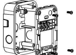
3F. COMPACT WALL MOUNT SURFACE-MOUNT BACK BOX
