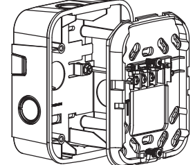
3B. WALL MOUNT SURFACE-MOUNT BACK BOX
