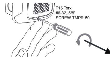
FIGURE 6. SURFACE MOUNT BACK BOX UP ARROW
