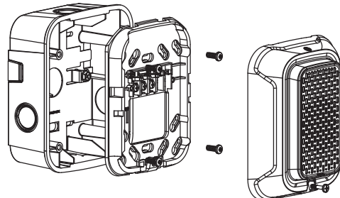
FIGURE 4. ATTACH DEVICE ONTO MOUNTING PLATE (SHOWN: WALL-MOUNT SOUNDER WITH SURFACE-MOUNT BACKBOX)
