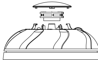
FIGURE 6: REMOVING/REPLACING SCREEN/SENSING CHAMBER
