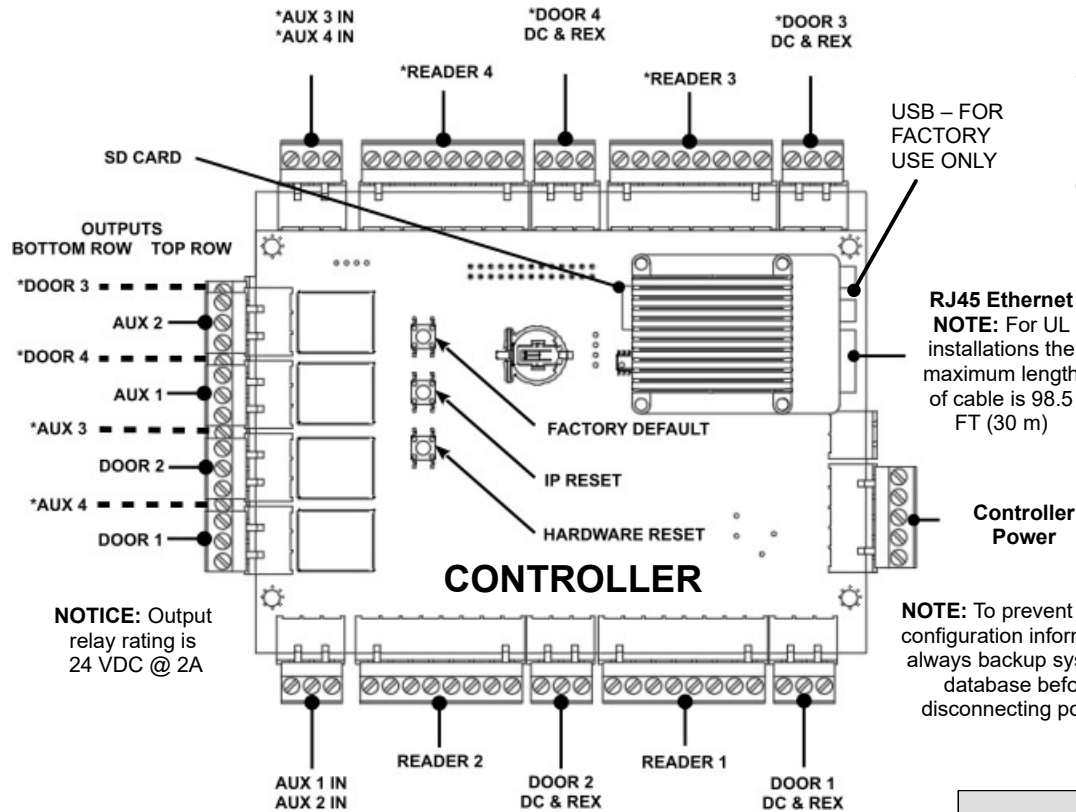
Controller Layout (*indicates only included on 4 Door models)
