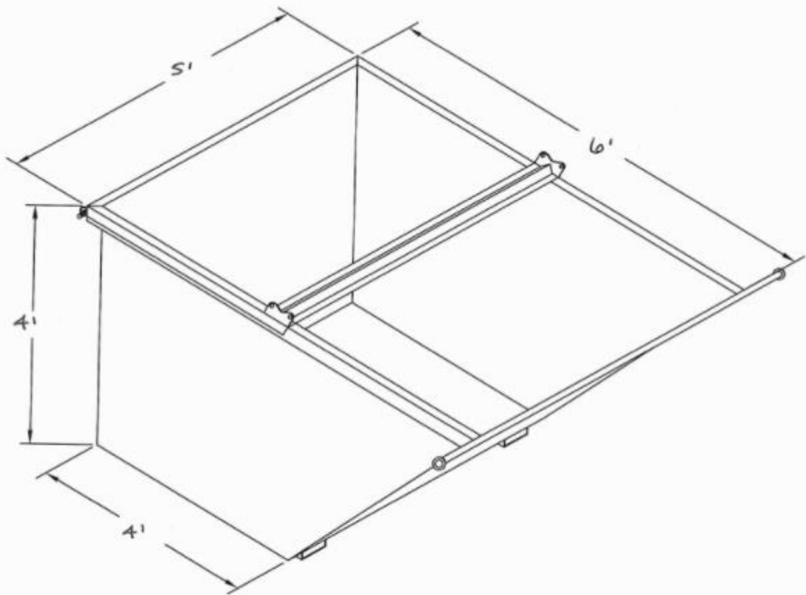
4 YARD REAR LOAD W/O CASTERS
