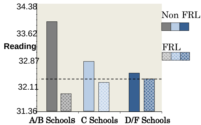
Figure 6. Graph from intercepts and slopes as outcomes model of Reading achievement. Results show lower average reading achievement for FRL students in A and B schools compared to C schools and D and F schools.
