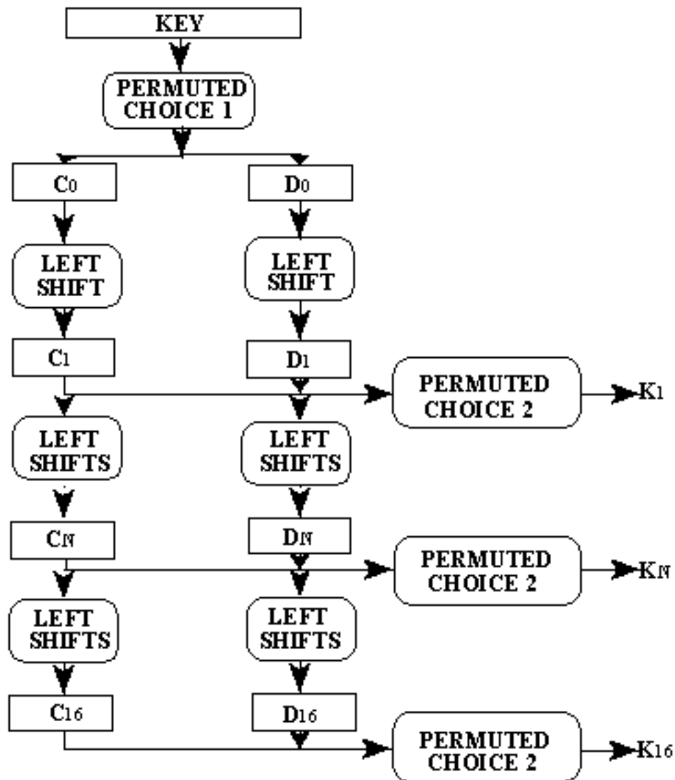
Figure 3. Key schedule calculation.
