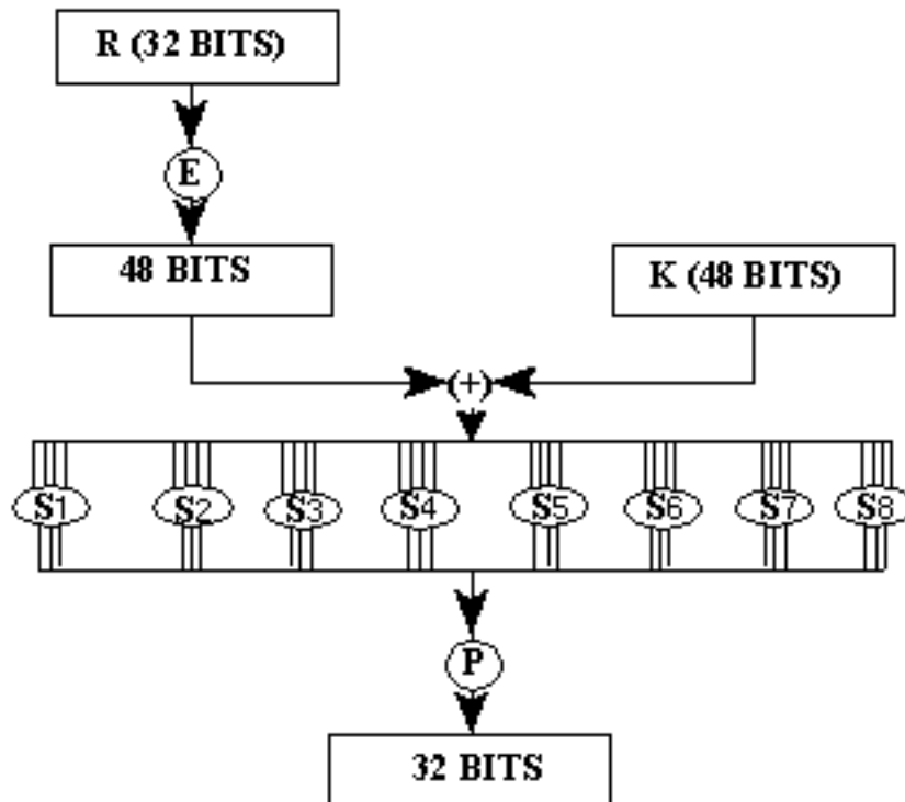
Figure 2. Calculation of f(R,K) .
