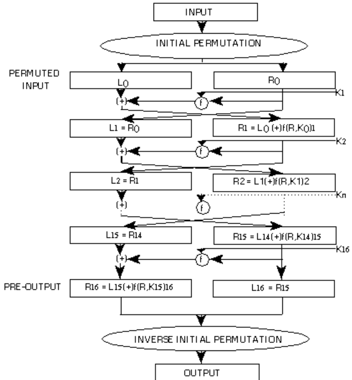
Figure 1. Enciphering computation.
