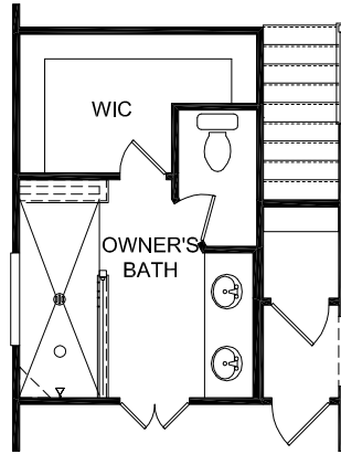
OPTIONAL OWNER'S BATH #3
