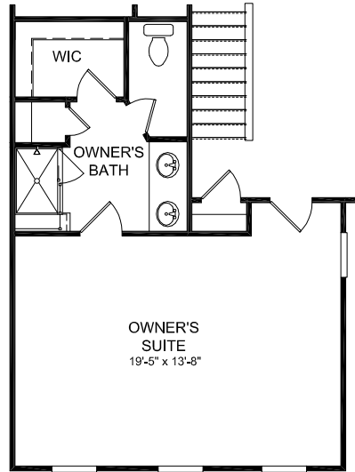
OPTIONAL SECOND OWNER'S SUITE
