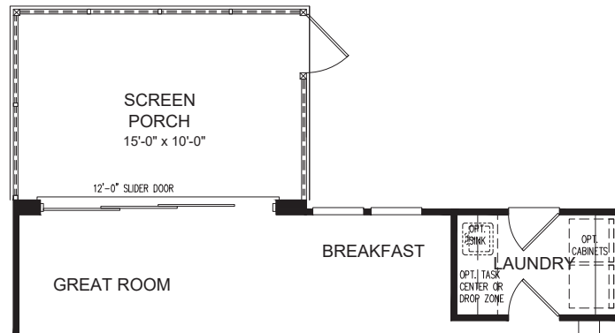
OPTIONAL SCREEN PORCH W/ OPT. REAR ENTRY DOOR 4
