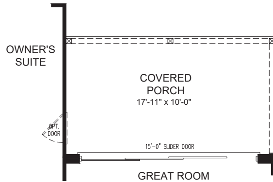
OPTIONAL COVERED PORCH W/ OPT. REAR ENTRY DOOR 4
