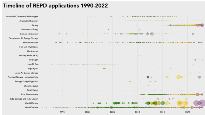
Figure 3. D3.js timeline
