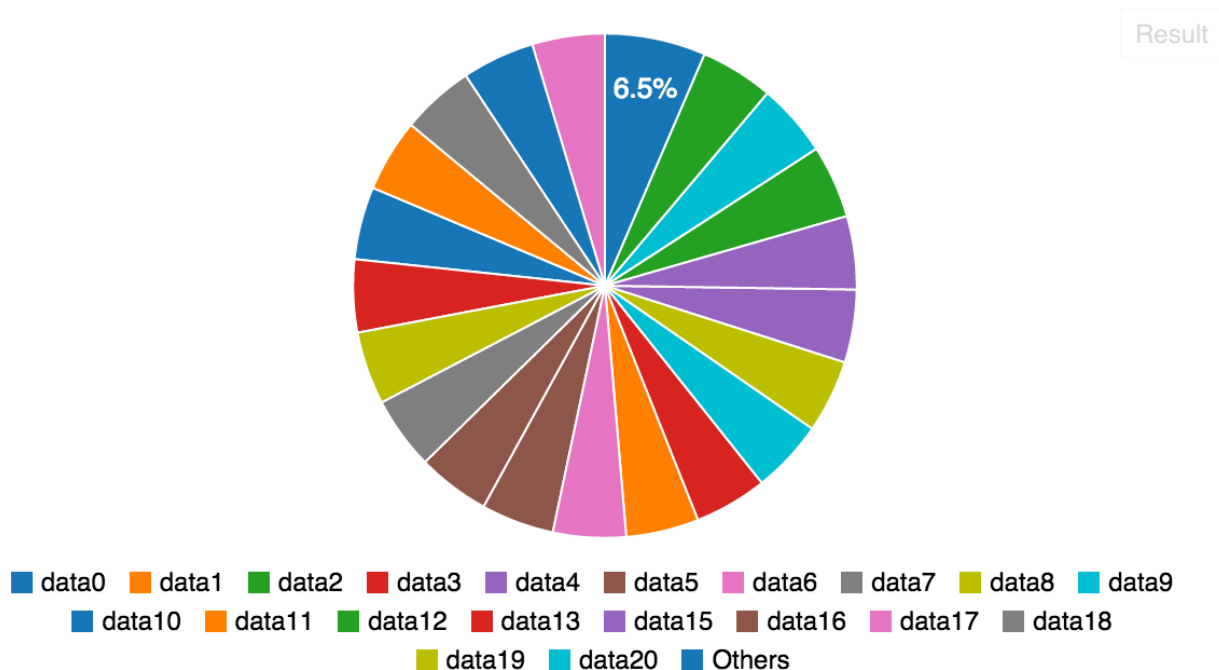
Pie chart with items merged
