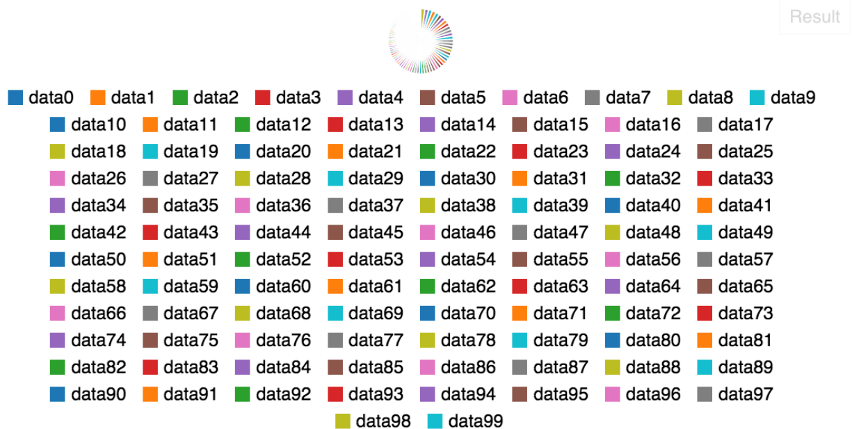
Unreadable pie chart with 100 items
