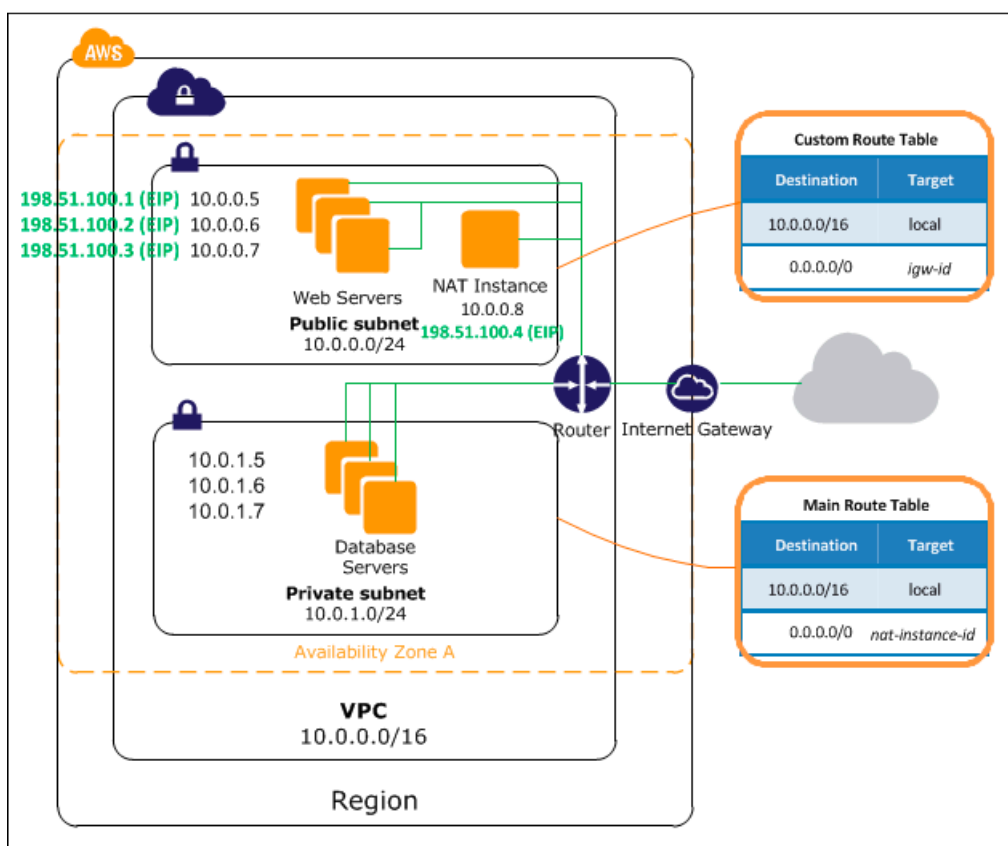
VPC Diagram
