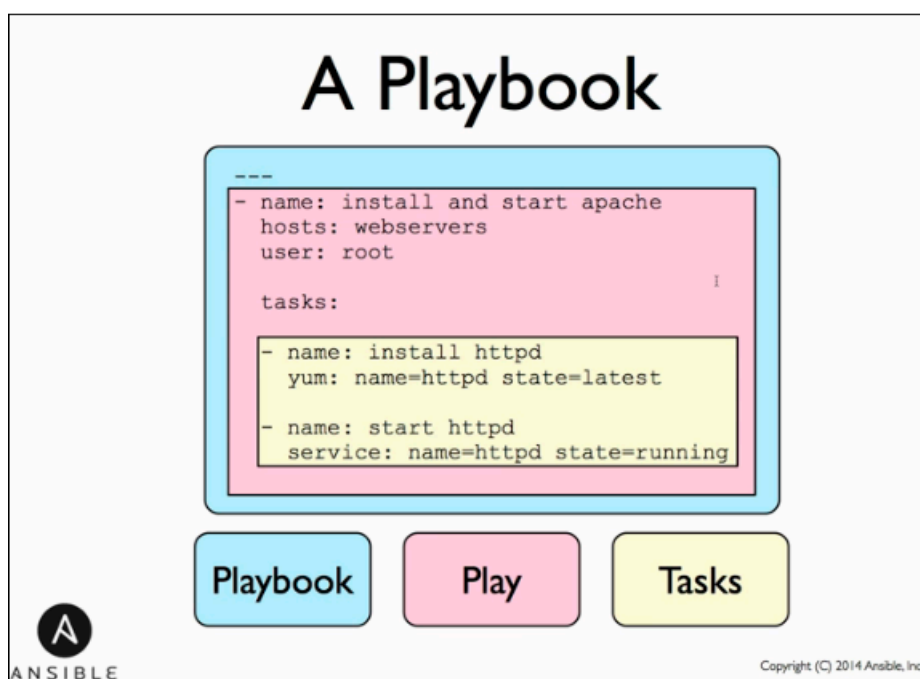
Ansible Playbook
