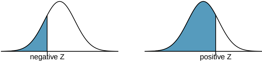
Figure C.2: The area to the left of Z represents the percentile of the observation.
