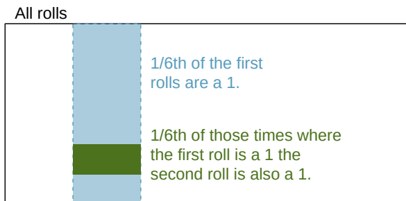
Figure 3.6: 1/6^{th} of the time, the first roll is a 1. Then 1/6^{th} of those times, the second roll will also be a 1.
