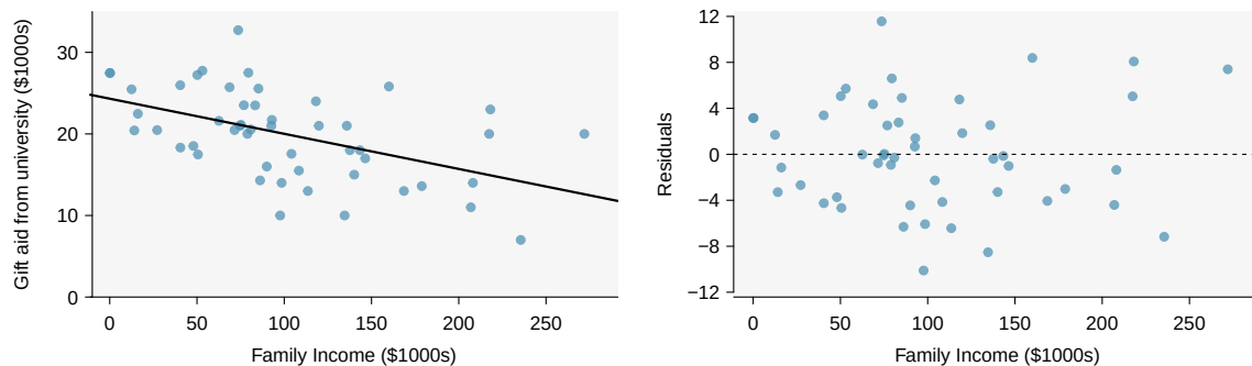
Figure 8.27: Left: Scatterplot of gift aid versus family income for 50 freshmen at Elmhurst college. Right: Residual plot for the model shown in left panel.
