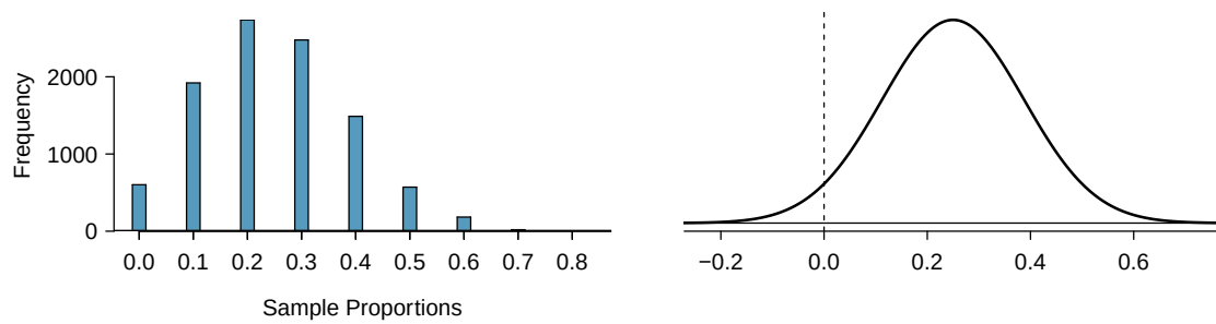
Figure 4.2: Left: simulations of \hat{p} when the sample size is n = 10 and the population proportion is p = 0.25 . Right: a normal distribution with the same mean (0.25) and standard deviation (0.137).
