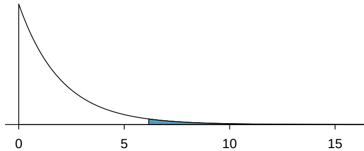
Figure 6.13: Computing the p-value for the Google hypothesis test.
