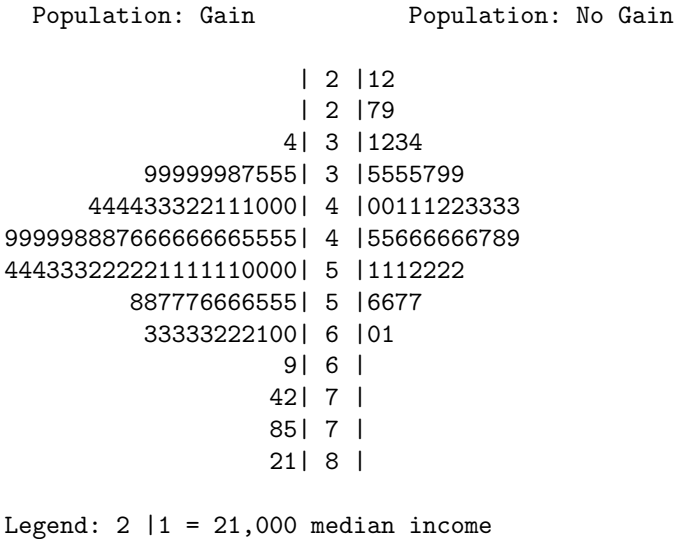
Figure 2.20: Back-to-back stem-and-leaf plot for median income, split by whether the count had a population gain or no gain.
