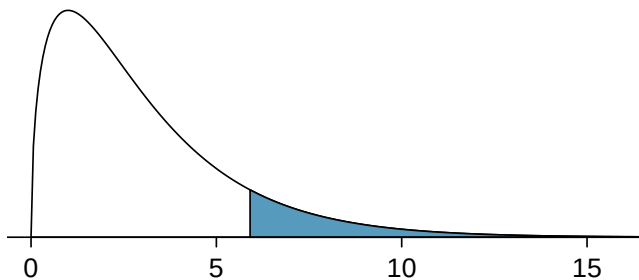
Figure 6.9: The p-value for the juror hypothesis test is shaded in the chi-square distribution with df = 3 .
