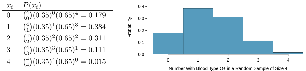
Figure 3.29: Probability distribution for the number with blood type O+ in a random sample of 4 people. This is a binomial distribution. Correcting for rounding error, the probabilities add up to 1, as they must for any probability distribution.
