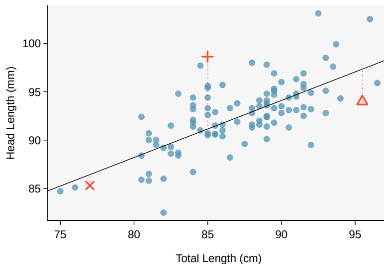
Figure 8.6: A reasonable linear model was fit to represent the relationship between head length and total length.
