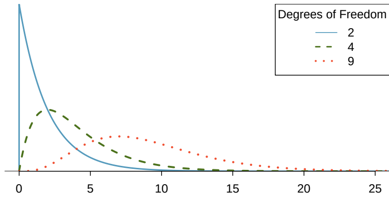
Figure 6.6: Three chi-square distributions with varying degrees of freedom.
