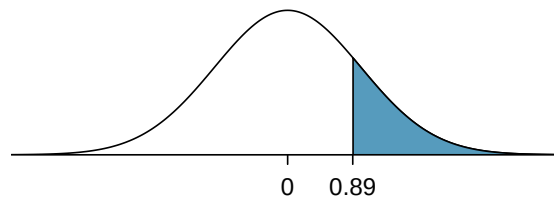
Figure 6.1: Sampling distribution for the sample proportion if the null hypothesis is true for Example 6.15. The p-value for the test is shaded.
