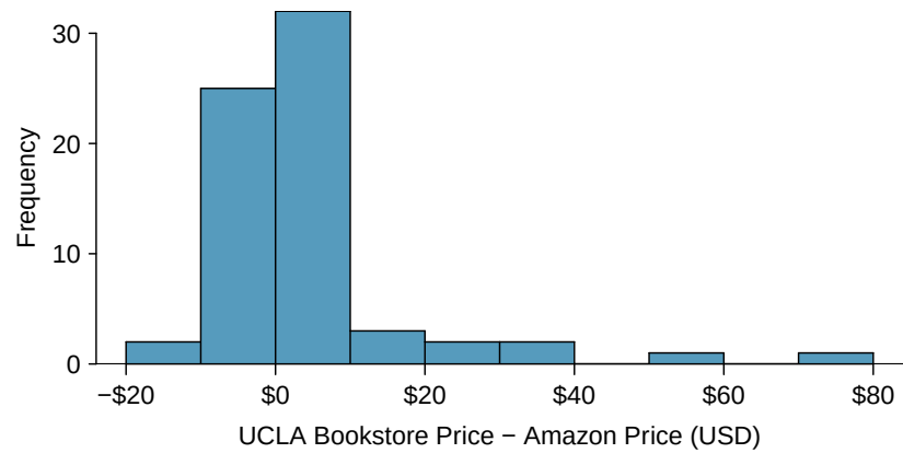
Figure 7.10: Histogram of the difference in price for each book sampled. These data are very strongly skewed. Explore this data set on Tableau Public + .
