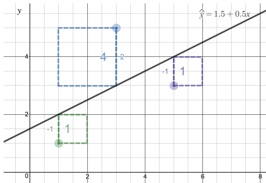
Figure 8.13: A visualization of least squares regression using Desmos. Try out this and other interactive Desmos activities at openintro.org/ahss/desmos .
