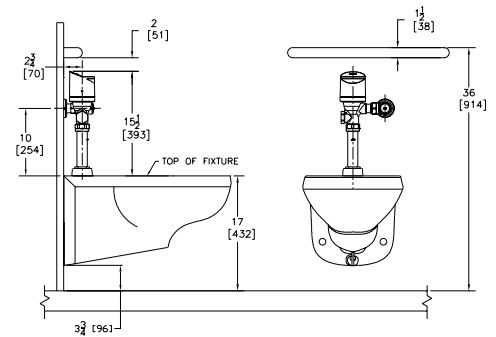
Water Closet Rough-in Dimensions
