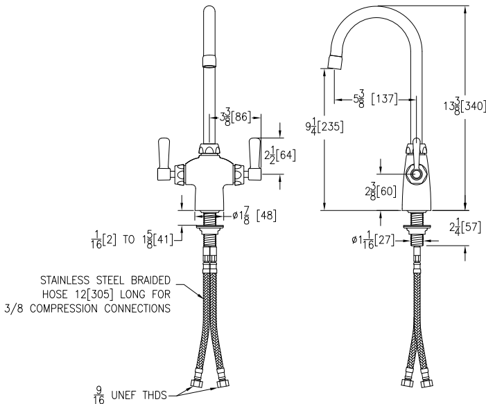
Rough-in/Overview dimensions
