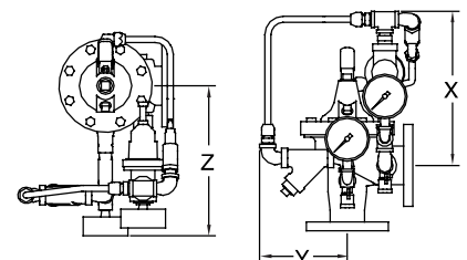
Angle Pilot System Dimensions
