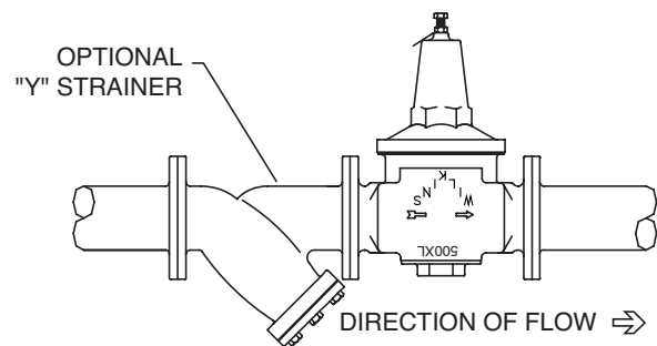
Horizontal Installation
