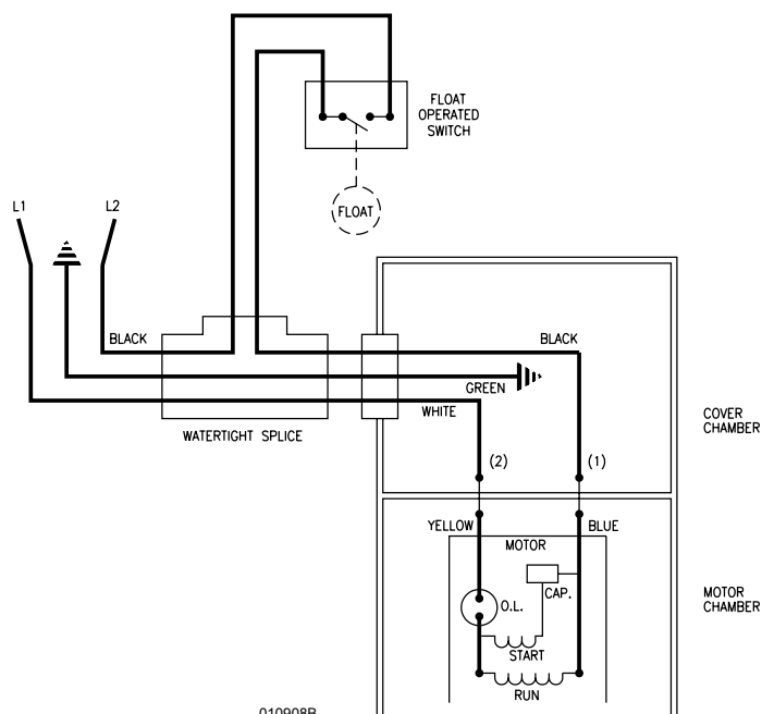
WIRING DIAGRAM FOR MODEL "WM152-A" 06/03 thru 10/06 "WM152-B" 11/06 thru Current
