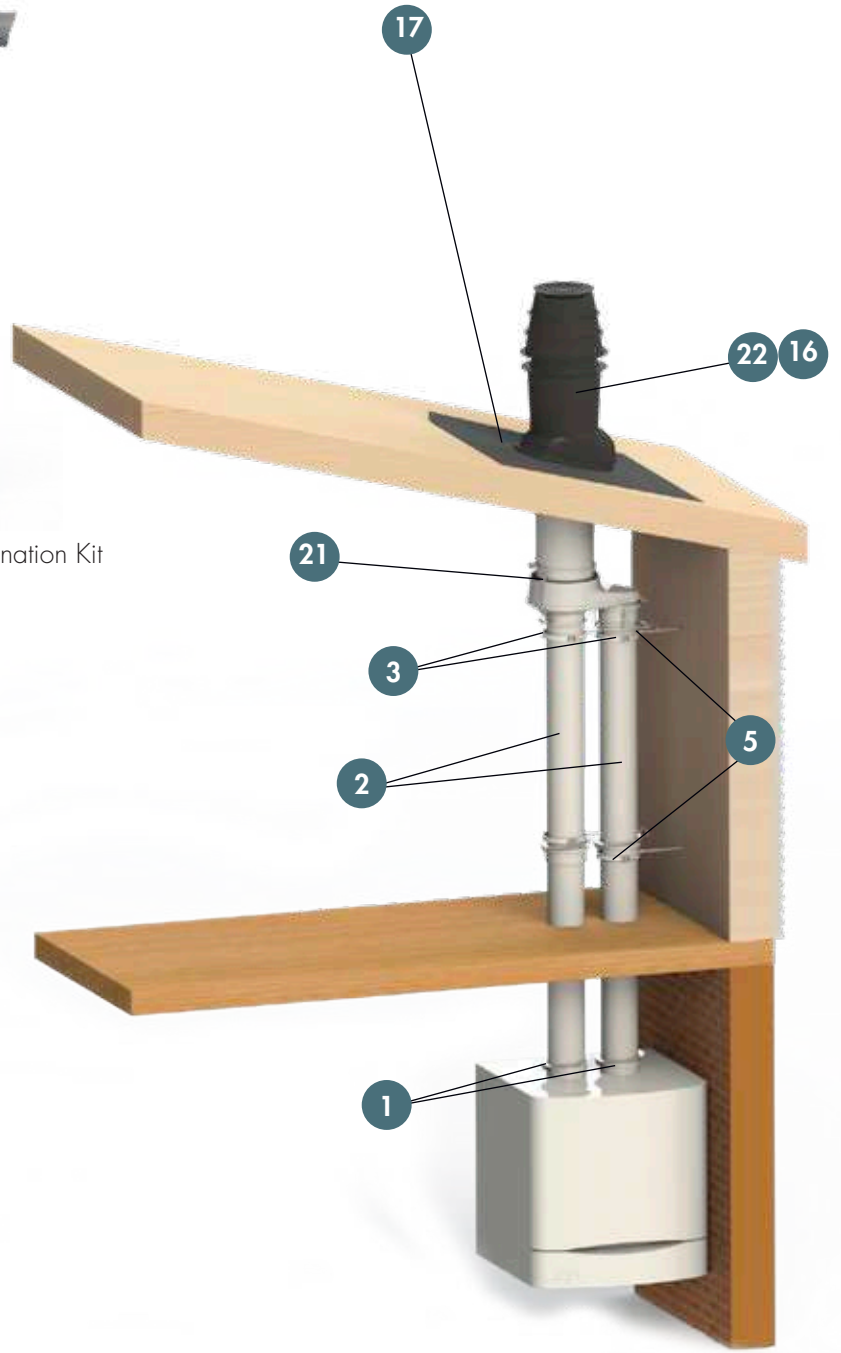
Vertical Vent and Air with Vertical Concentric Termination Kit
