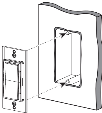
Wallbox Mount
