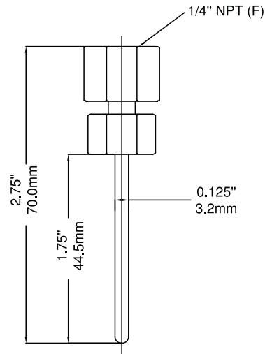
Gauge Adaptor 2.75"
