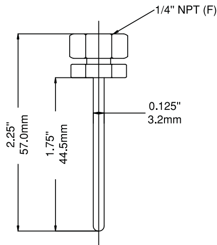
Gauge Adaptor 2.25"
