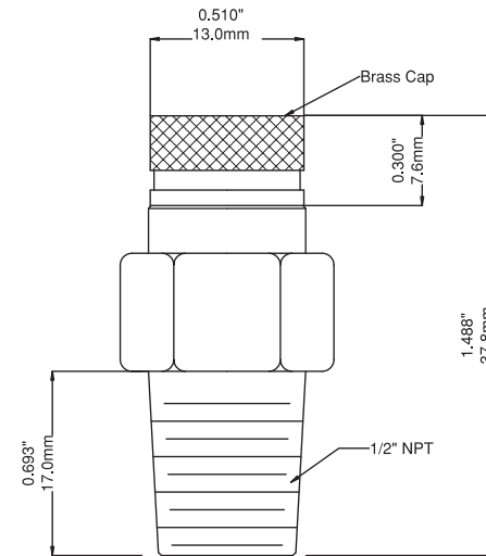
0.5" Test Plug
