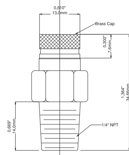
0.25" Test Plug
