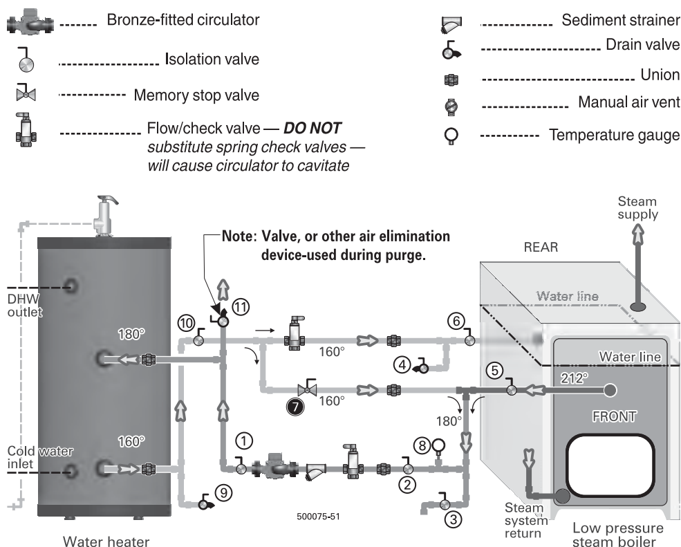
Figure 16 Low pressure steam boiler application — Domestic water heating using water pumped from steam boiler
