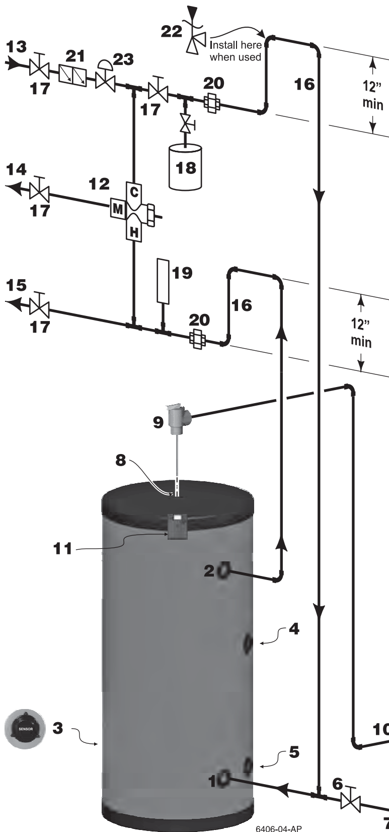
Figure 2 DHW piping
