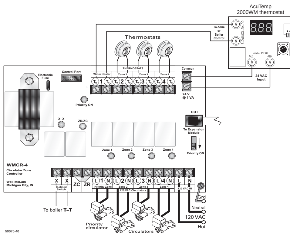
Figure 25 Typical wiring — zoning with circulators — DHW priority with Weil-McLain WMCR Circulator Zone Controller
