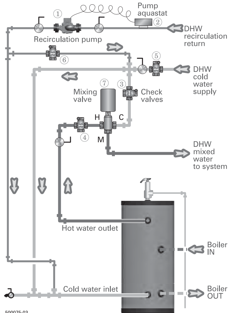
Figure 6 Recirculation piping
