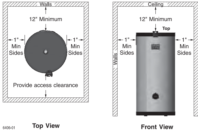
Figure 1 Clearance recommendations
