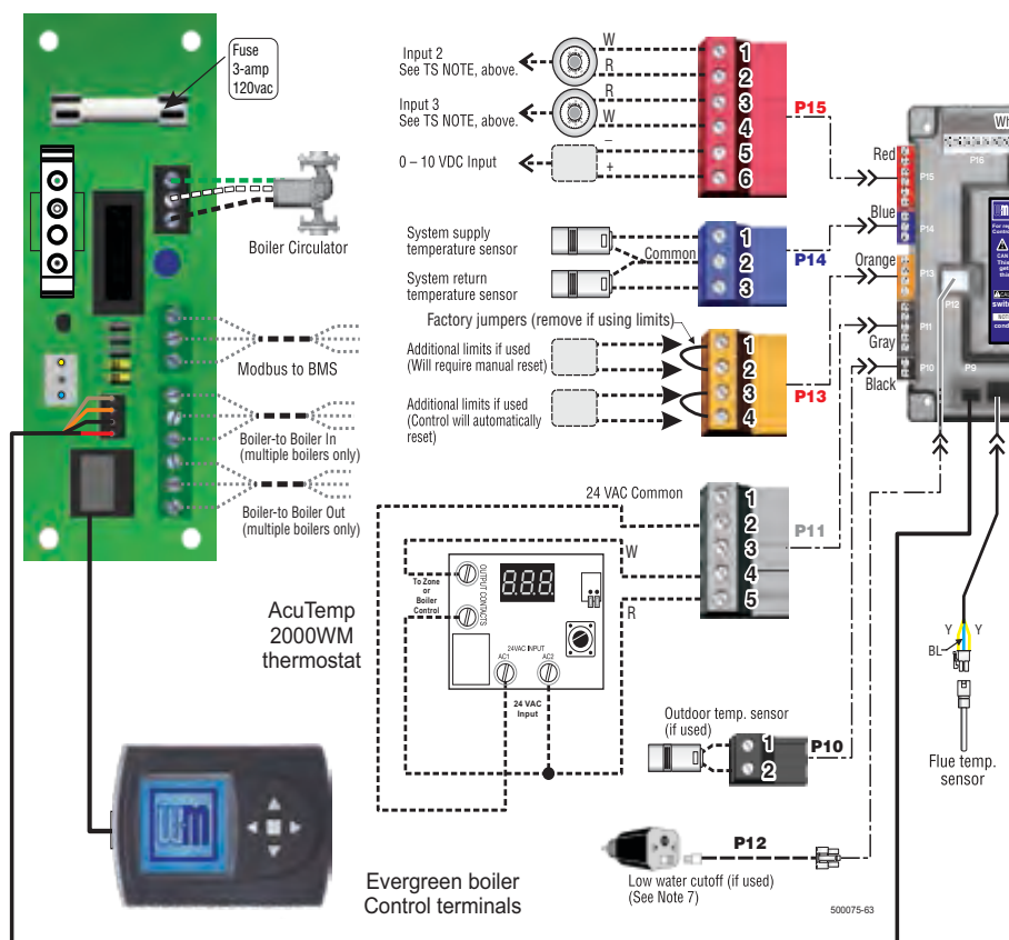
Figure 21 Wiring the control to the Evergreen (1176-160) and SlimFit 550-750 (1176-170) boiler controls will connect to the AcuTemp 2000WM thermostat.
