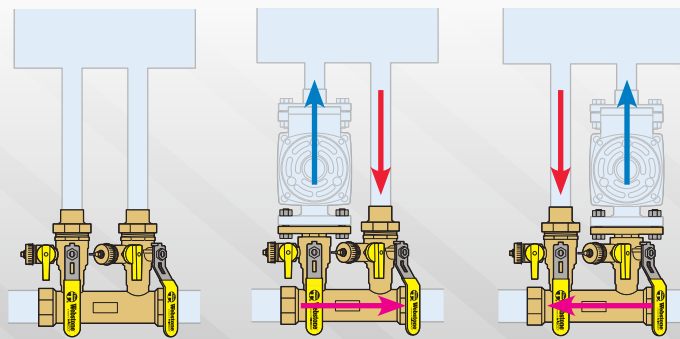
PUMP INTERNAL TO BOILER Double Ball Drain Manifold
