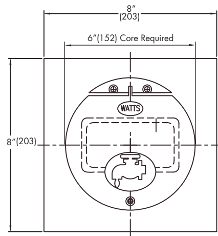
-R Round Box for Tilt-Up Construction
