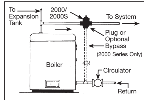
Horizontal Installation
