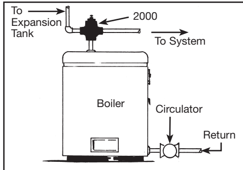
Angle Installation
