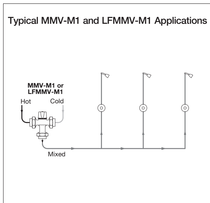
Figure 1 – Typical ASSE 1069 Application
