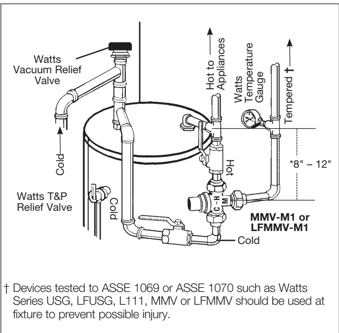
Figure 3 – Typical ASSE 1017 Application
