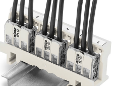
Mounting type (440 V) Vertical mounting on DIN-35 rail
