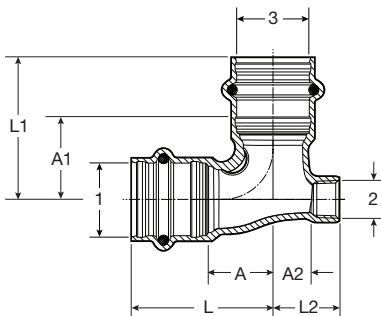
Vieg ProPress Vent Tee Zero Lead Bronze P x FPT x P - Model 2917.3ZL
