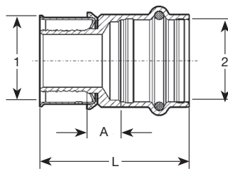
Viega PEX Press Adapter Zero Lead Bronze P x P - Model 2813PZL
