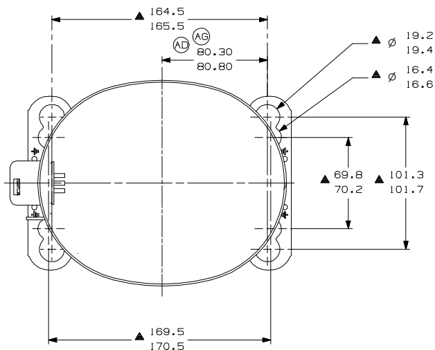
- AUXILIARY VIEW - FASTENING DIMENSIONS
