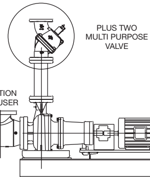
BASE MOUNTED SINGLE SUCTION PUMP
