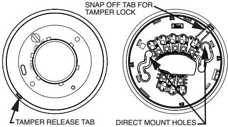
FIGURE 2: TAMPER-RESISTANT FEATURE
