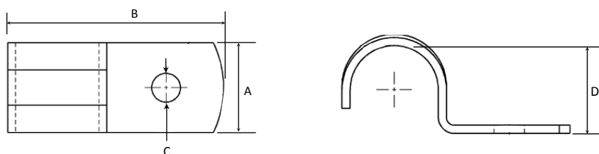
One-hole straps – steel/zinc plated
