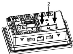
2 RTC battery case
