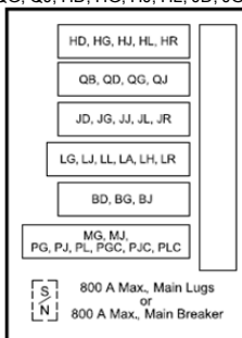
TYPE HCP-SU 800 A max. main circuit breaker 600 A max. branch circuit breaker BD, BG, BJ, LA, LG, LJ, LL, LH, LR, MG, MJ, PG, PJ, PL, PGC, PJC, PLC [2] , QB, QD, QG, QJ, HD, HG, HJ, HL, JD, JG, JJ, JL
