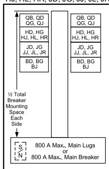
TYPE HCP-SU 800 A max. main circuit breaker 600 A max. branch circuit breaker BD, BG, BJ, LA, LG, LJ, LL, LH, LR, MG, MJ, PG, PJ, PL, PGC, PJC, PLC [2] , QB, QD, QG, QJ, HD, HG, HJ, HL, JD, JG, JJ, JL
