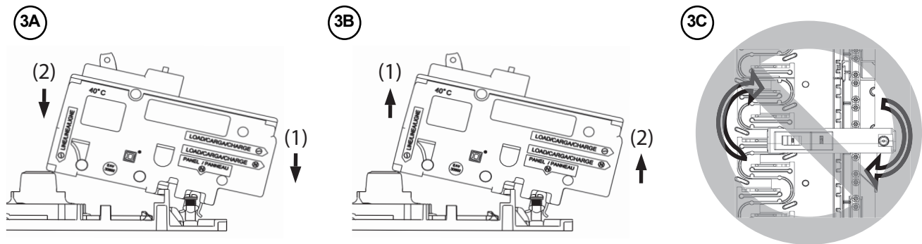
Figure / Figura / Figure 3 : Removal / Desmontaje / Retrait
