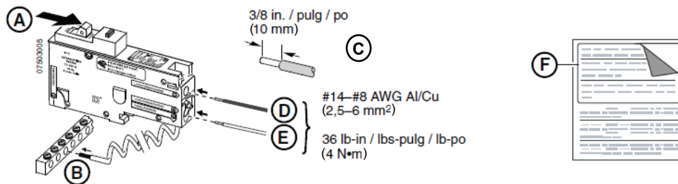
Figure / Figura / Figure 1 : Installation / Instalación / Installation
