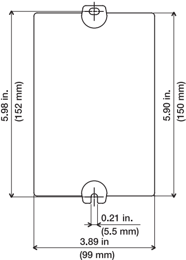
30 A Enclosed Switch Mounting Diagram
