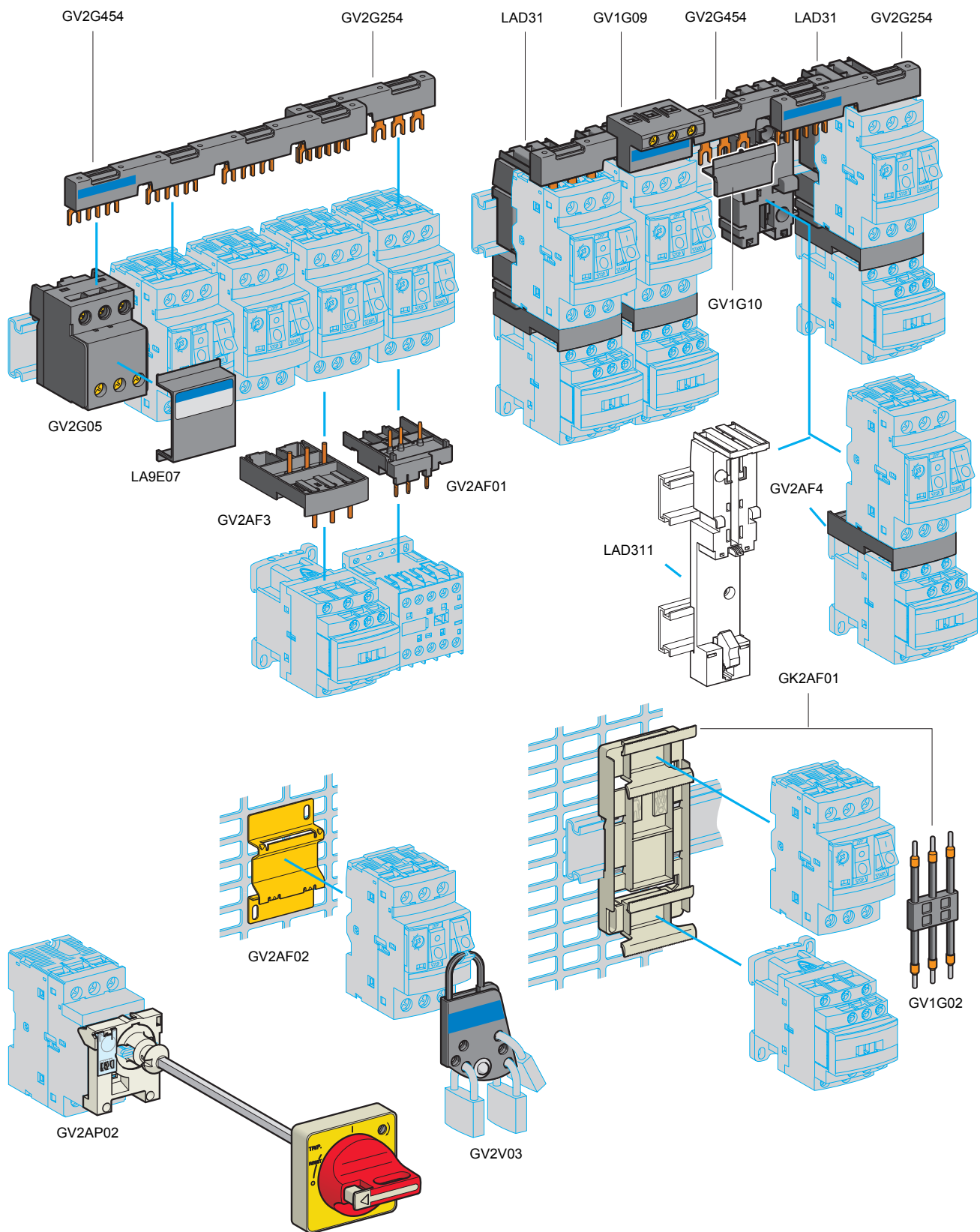
Figure 3: GV2 Accessories
