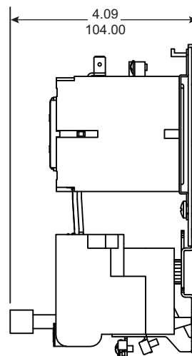
Figure 9: Approximate Dimensions
