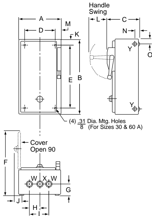
Figure 16.23: NEMA 1 Enclosure, Combination Devices
