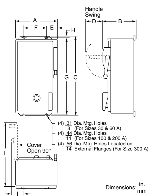
Figure 16.26: NEMA 12/3R Enclosure
