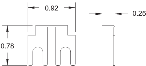
Jumper
