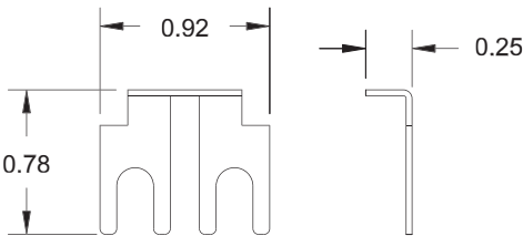
Jumper
