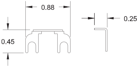
Jumper
