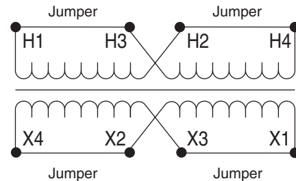
Parallel Connections
