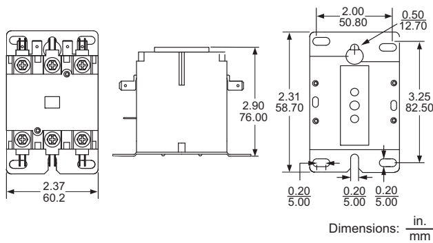
Figure 5: Type DPA, 2 and 3 Pole 20–40 Full Load Amperes
