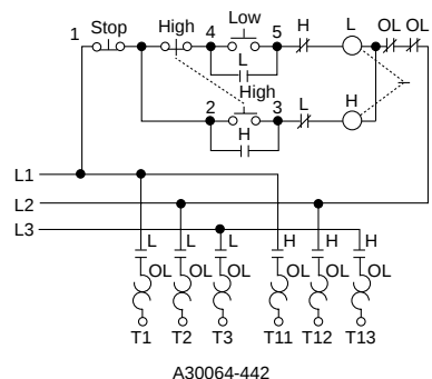
A30064-442 2-Speed Separate Winding Constant HP, Constant Torque and Variable Torque NEMA Size 0-4 Sizes 5, 6 & 7 Use Special Circuitry
